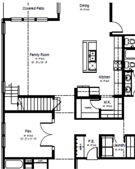
Opt. Bonus Room Partial Main Floor Plan
