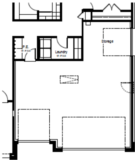
Opt. Garage Storage Partial Main Floor Plan
