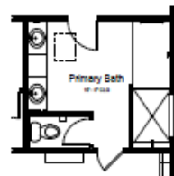
Opt. Primary Bath Super Shower Partial Main Floor Plan
