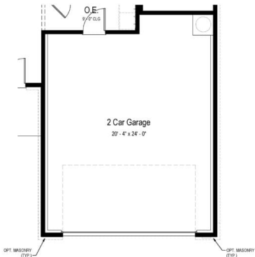
Opt. 4' Garage Extension Partial Main Floor Plan SCALE: 1/8" = 1'-0" (+84 Sq. Ft)
