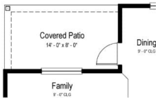
Opt. Covered Patio Partial Main Floor Plan SCALE: 1/8" = 1'-0"
