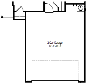
Opt. 4' Garage Extension Partial Main Floor Plan
