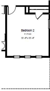
Opt. 4' Garage Extension Partial Upper Floor Plan
