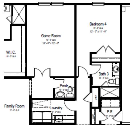
Opt. Bedroom 4 Suite w/ Powder Bath Partial Main Floor Plan
