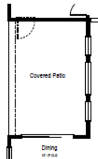
Opt. SGD @ Dining Partial Main Floor Plan
