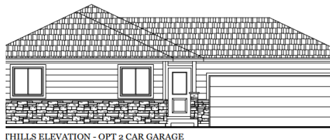
THILLS ELEVATION - OPT 2 CAR GARAGE
