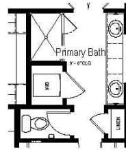
Opt. Primary Bath Drawer Base ILO Kneespace Partial Main Floor Plan
