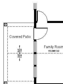
Opt. Covered Patio Partial Main Floor Plan
