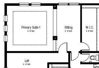
Opt. Primary Suite Relax V1 Partial Upper Floor Plan
