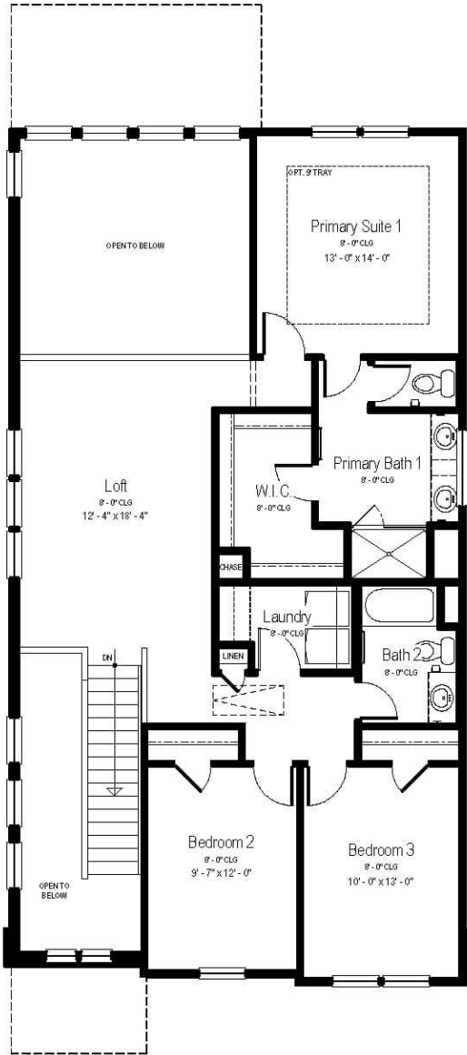
UPPER FLOOR
