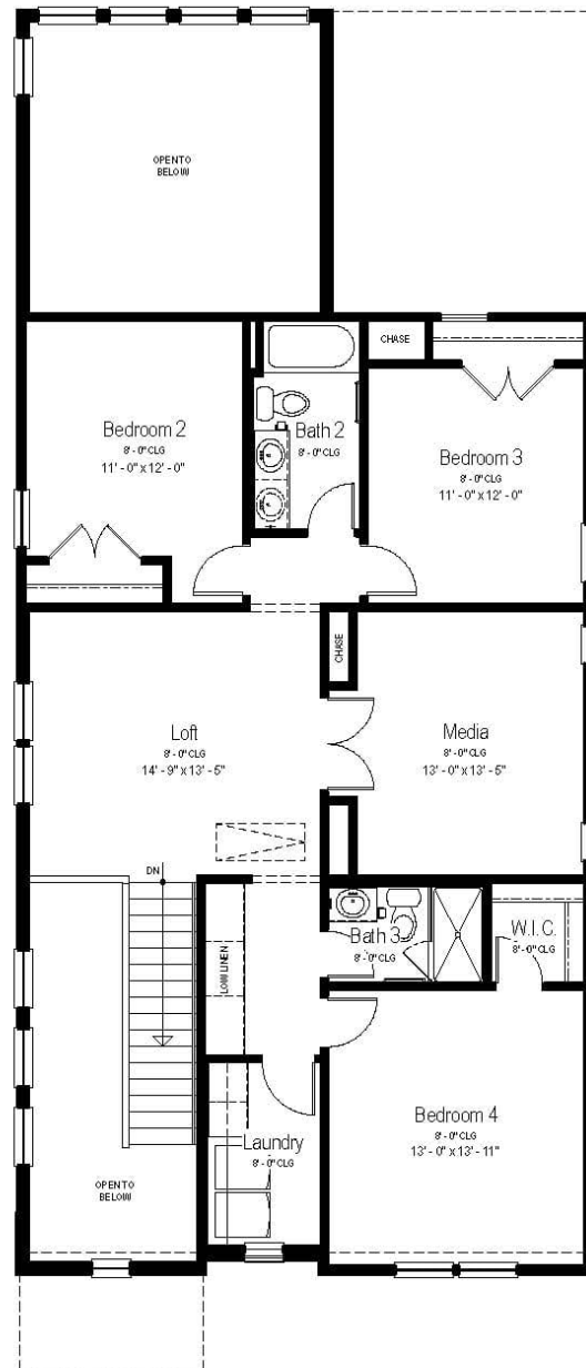
UPPER FLOOR
