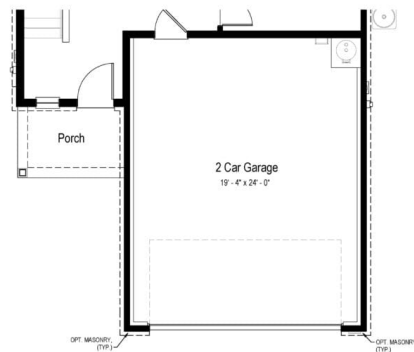
Opt. 4' Garage Extension Partial Main Floor Plan
