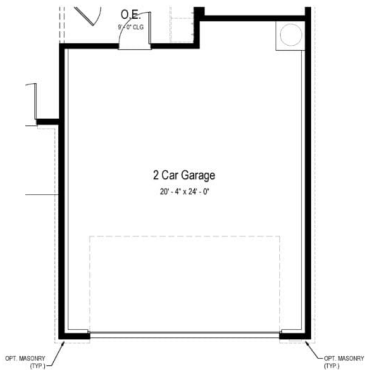
Opt. 4' Garage Extension Partial Main Floor Plan (+84 Sq. Ft.)
