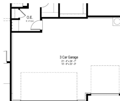
Opt. 3 Car Garage Partial Main Floor Plan
