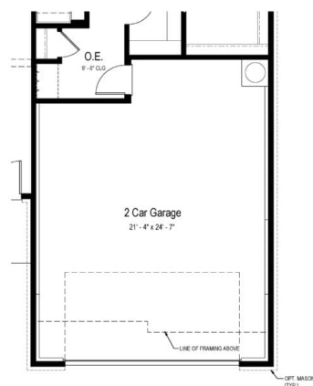
Opt. 4'-0" Garage Extension Partial Main Floor Plan
