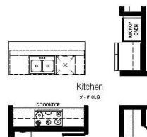
Opt. Gourmet Kitchen Partial Main Floor Plan
