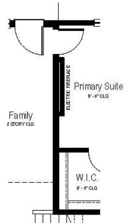
Opt. Fireplace at Primary Partial Main Floor Plan
