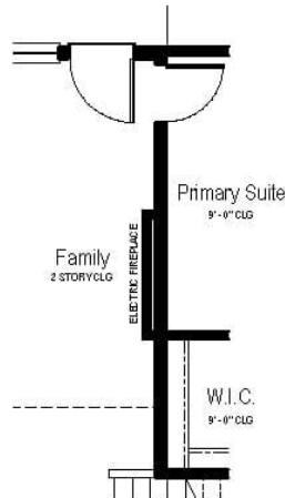
Opt. Fireplace @ Family Partial Main Floor Plan
