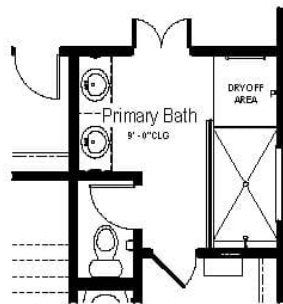
Opt. Super Shower Partial Main Floor Plan
