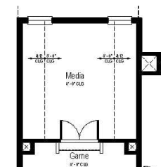
Opt. Media Room Partial Upper Floor Plan
