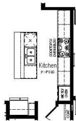
Opt. Chef Kitchen Partial Main Floor Plan
