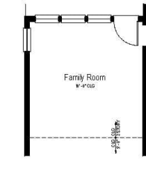
Opt. Media Room Partial Main Floor Plan
