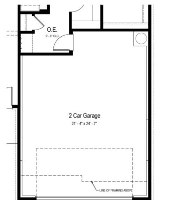
Opt. 4'-0" Garage Extension Partial Main Floor Plan
